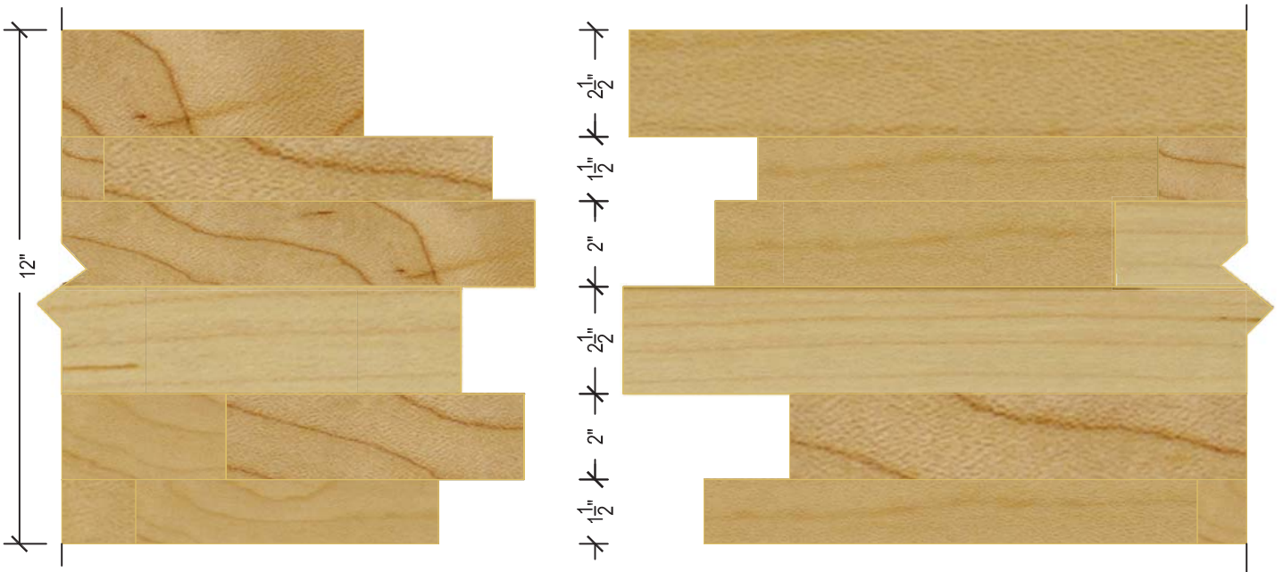
(scale 3" = 1')
