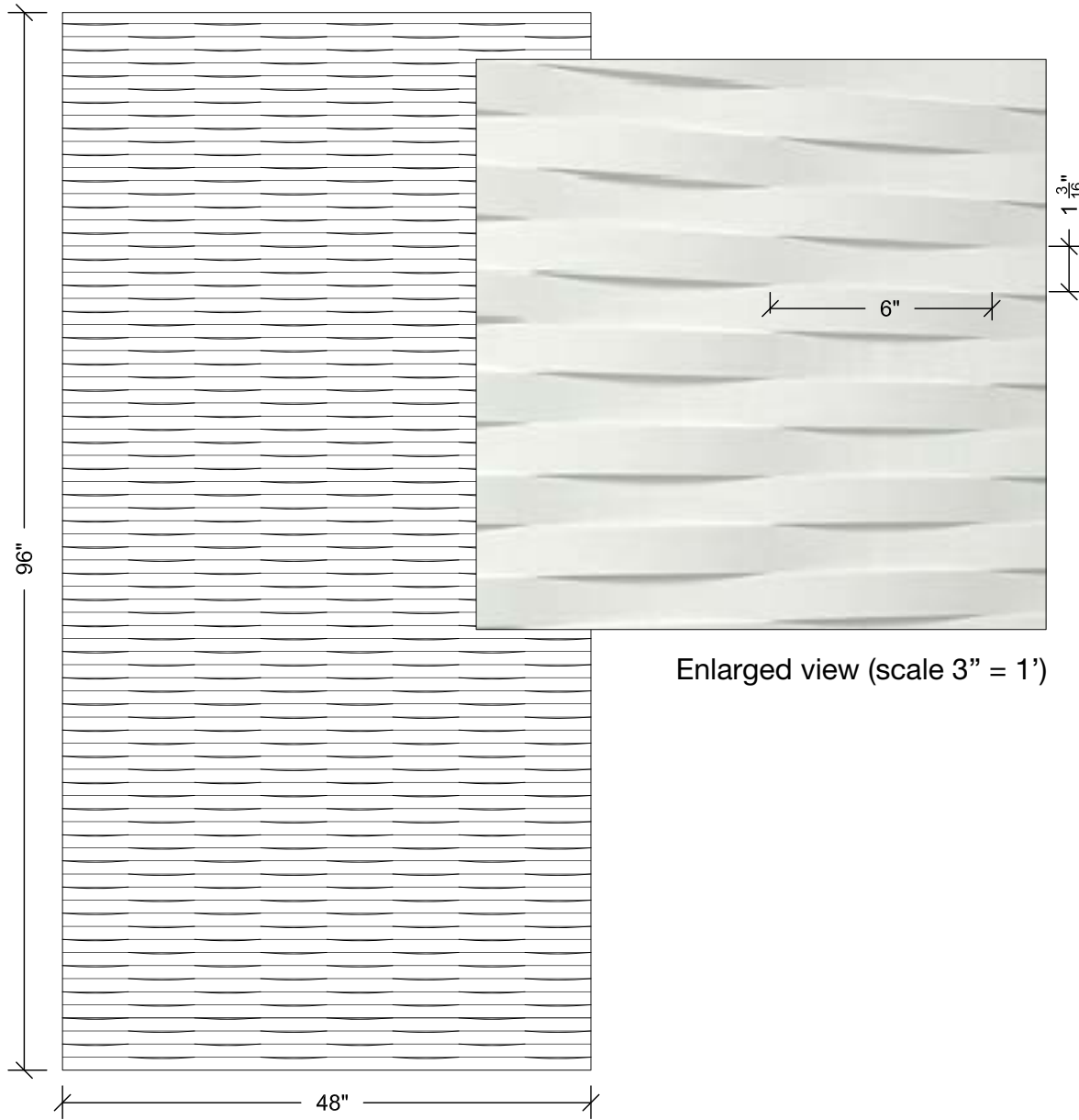
WPMAS009 (scale 3/4" = 1')
